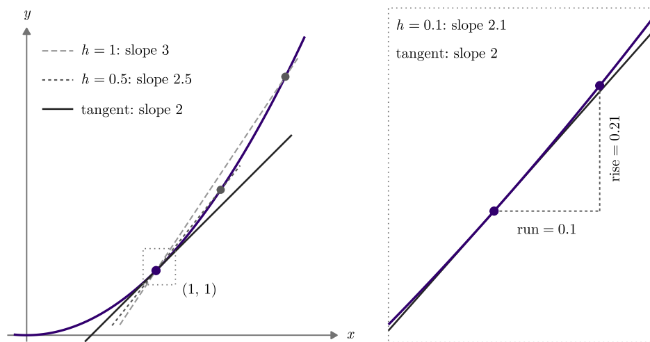
Figure 1.6: The derivative of f(x) = x^2 at x = 1 . Left: lines through (1, 1) and (1 + h, (1 + h)^2) have slope 2 + h .
