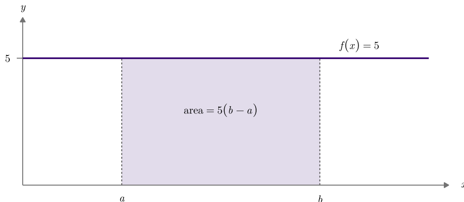
Figure 1.7: The integral of the constant function f(x) = 5 from a to b is the shaded rectangle, with area 5(b - a) .
