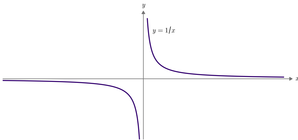
Figure 1.5: The limit of 1/x as x \rightarrow \infty or x \rightarrow -\infty is 0.
