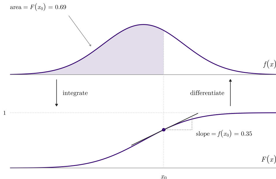
Figure 1.8: Differentiation and integration are one relationship read in two directions. Integrating the density f up to x_0 gives the area F(x_0) = P(X \leq x_0) ; differentiating F at x_0 gives back the height f(x_0) , which is the slope.
