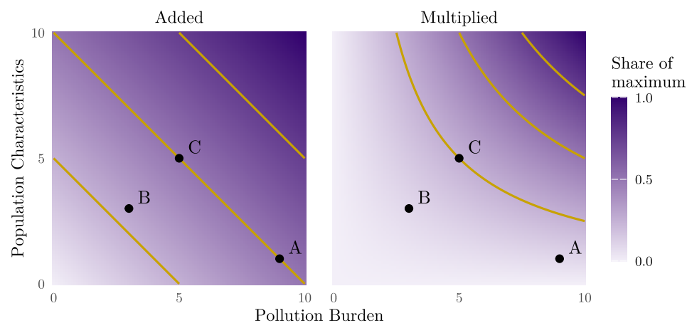
Figure 3.4: The score for every combination of the two components, each on a 0 to 10 scale.
