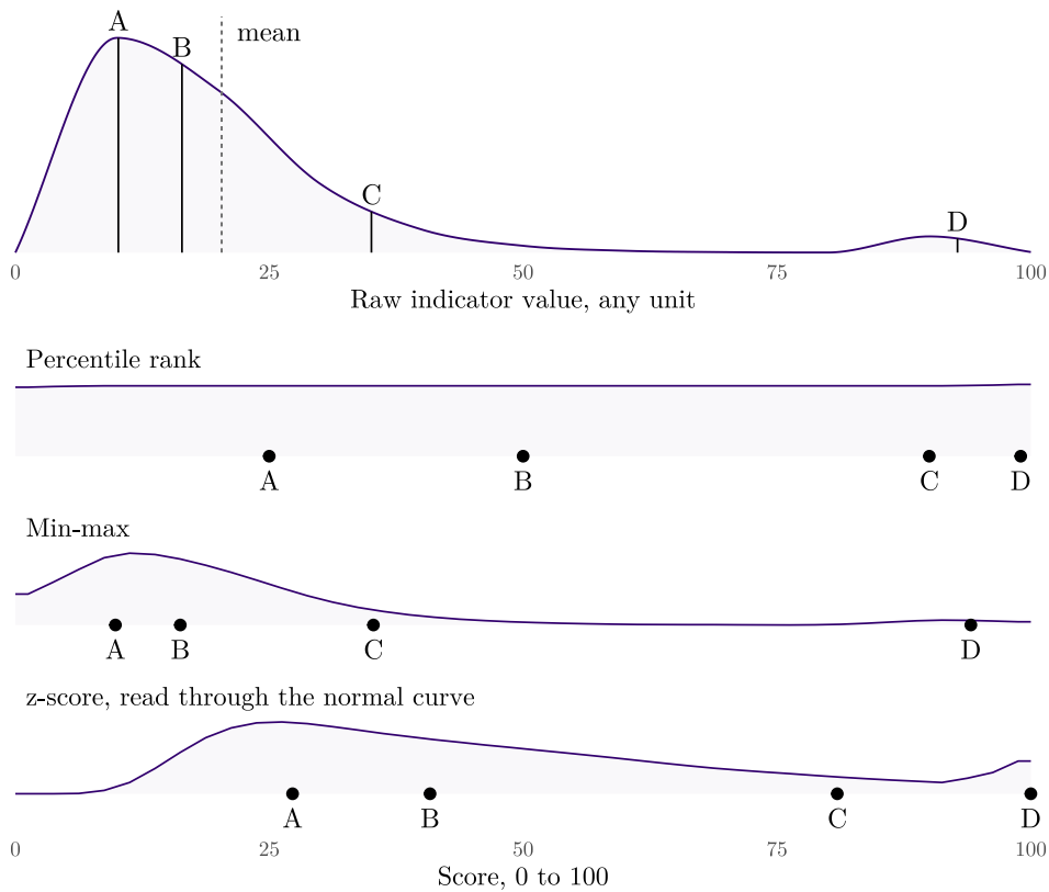
Figure 3.2: The same 1,000 simulated tracts standardized in three ways, each on a 0 to 100 scale.
