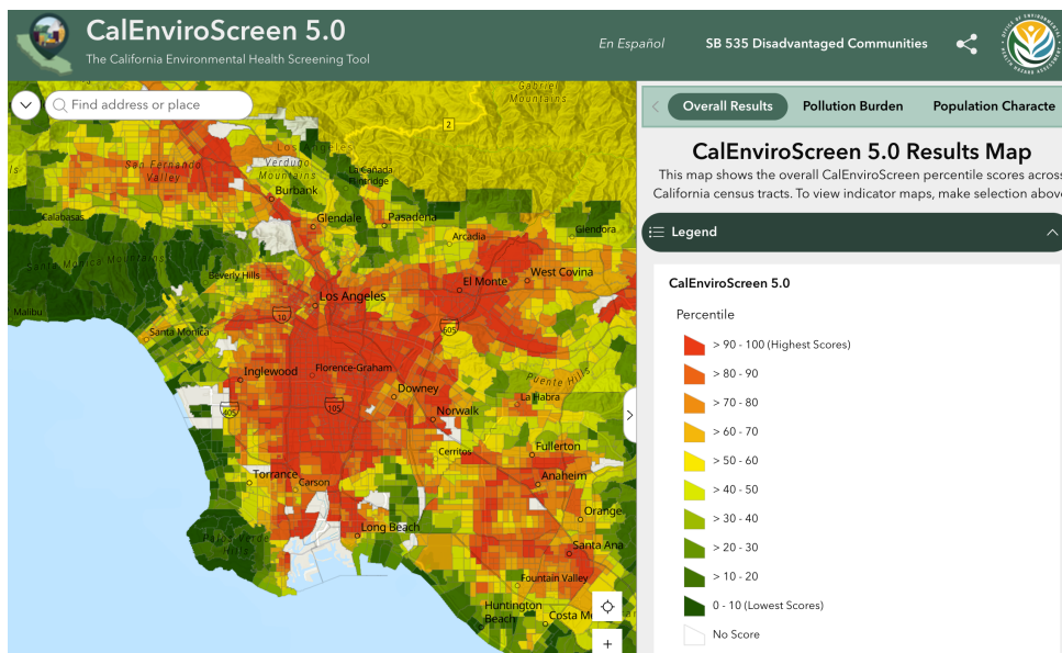
Figure 3.1: CalEnviroScreen 5.0
